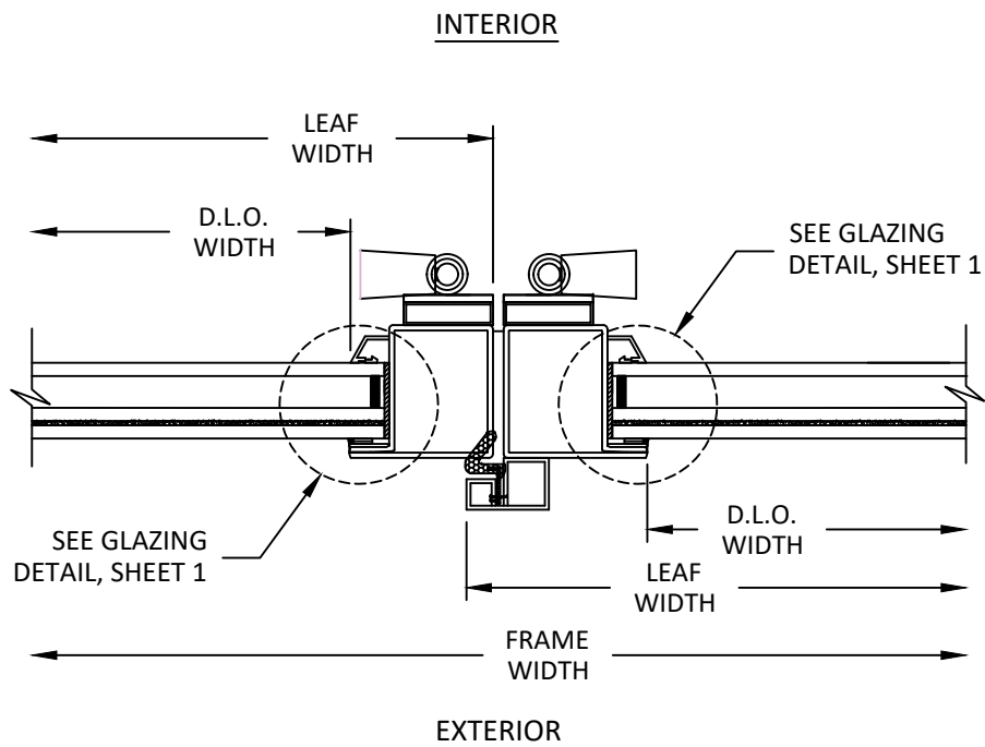
E 8 HORIZONTAL SECTION ASTRAGAL
