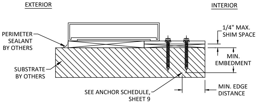
C 10 VERTICAL SECTION SIDELITE SILL - NAIL FIN INSTALLATION
