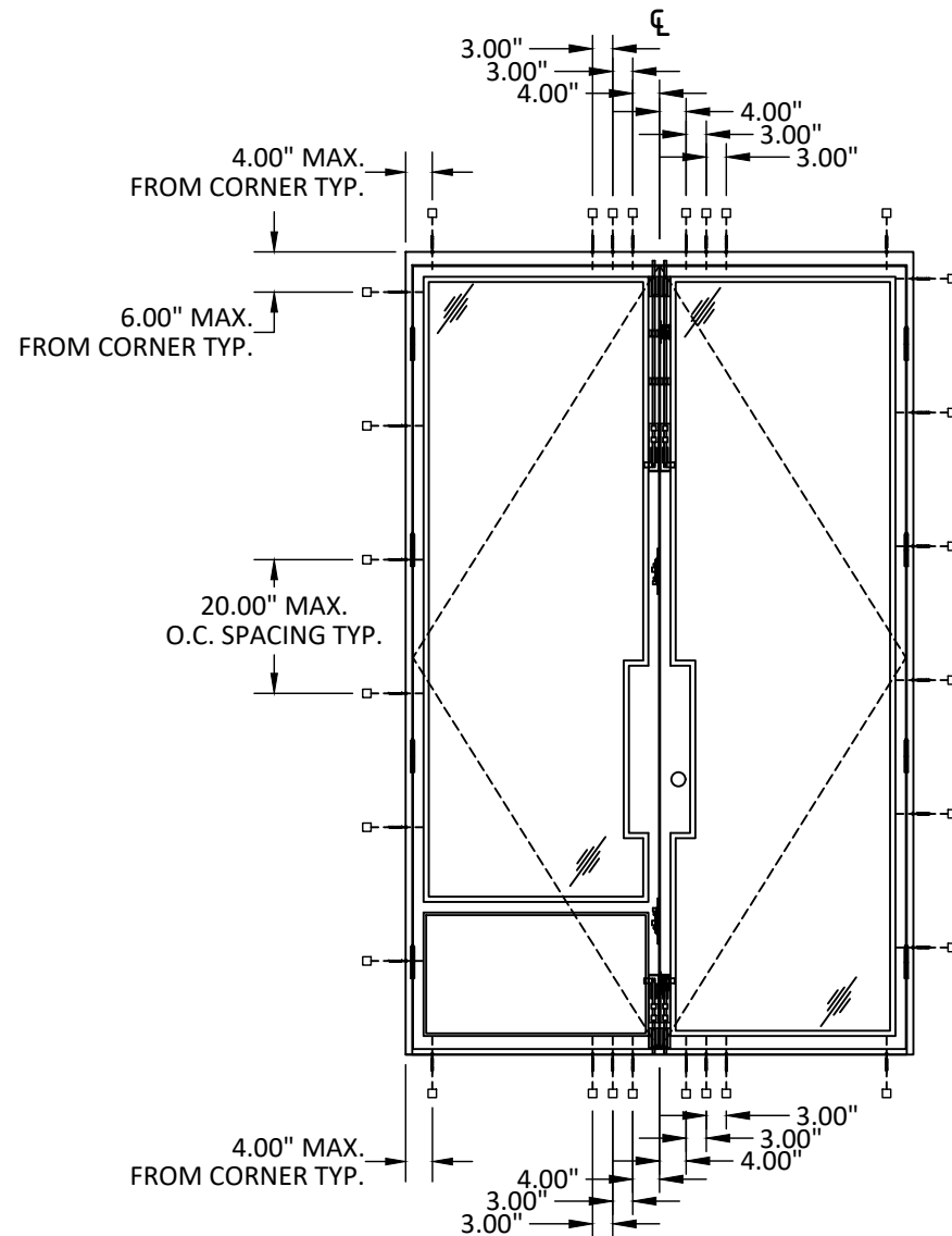
ANCHOR LAYOUT FRENCH DOOR THROUGH FRAME INSTALLATION
