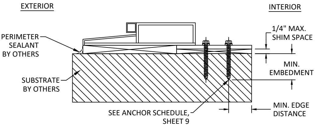
B 10 VERTICAL SECTION DOOR SILL - TAB INSTALLATION
