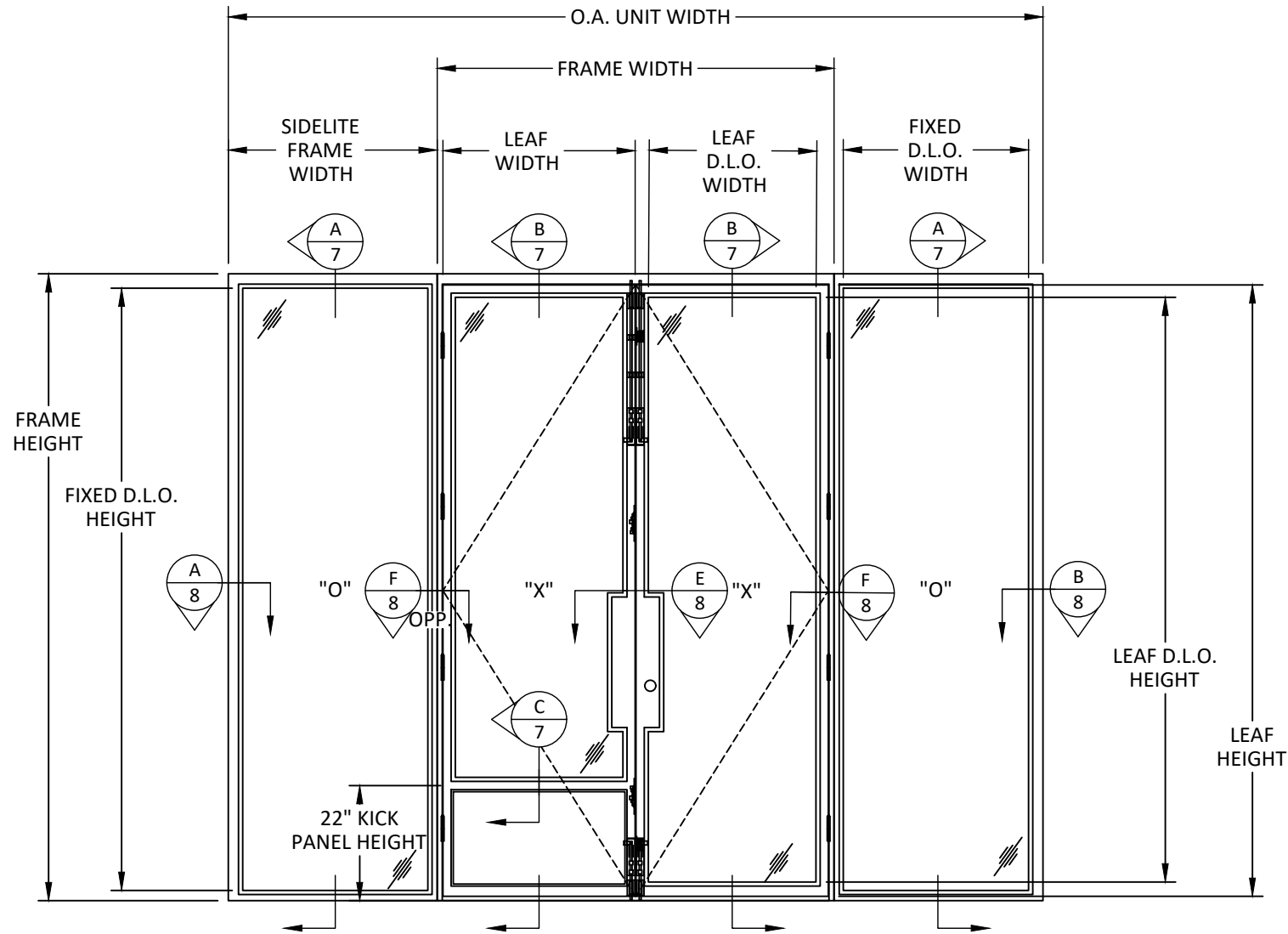
ELEVATION FRENCH DOOR WITH SIDELITES
