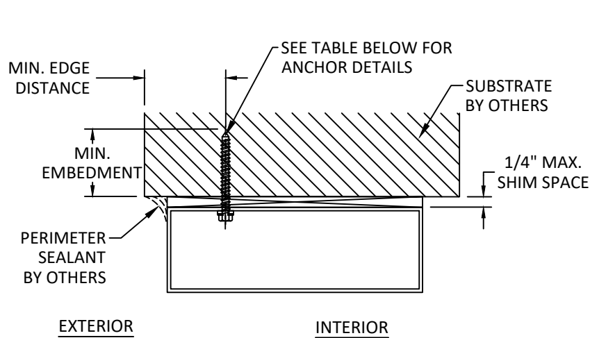
A 9 VERTICAL SECTION DOOR HEAD - THROUGH FRAME INSTALLATION
