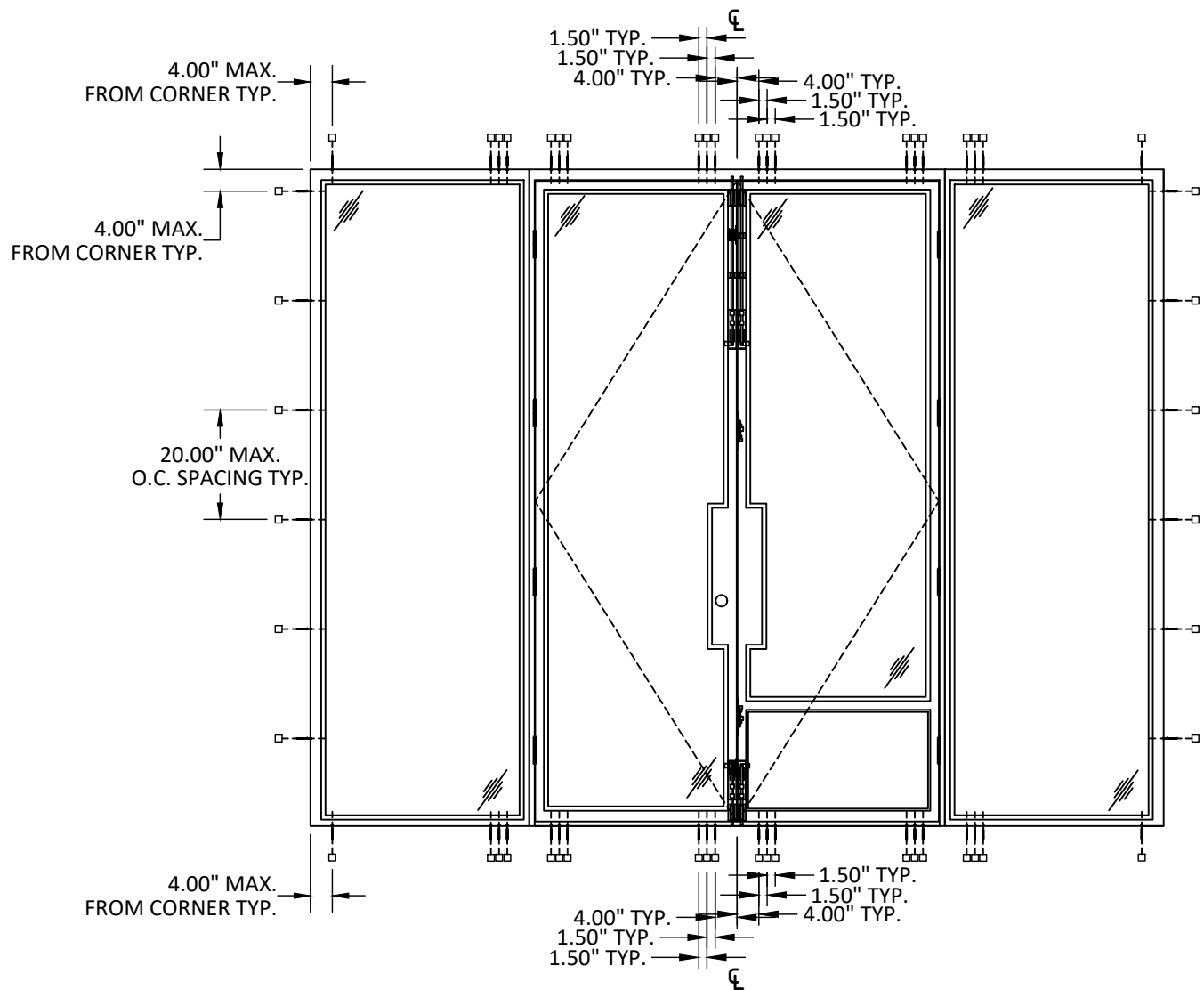
ANCHOR LAYOUT FRENCH DOOR WITH SIDELITES THROUGH FRAME INSTALLATION
