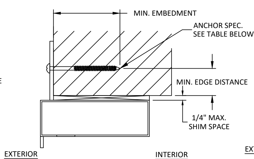
B 9 VERTICAL SECTION SIDELITE HEAD - NAIL FIN INSTALLATION
