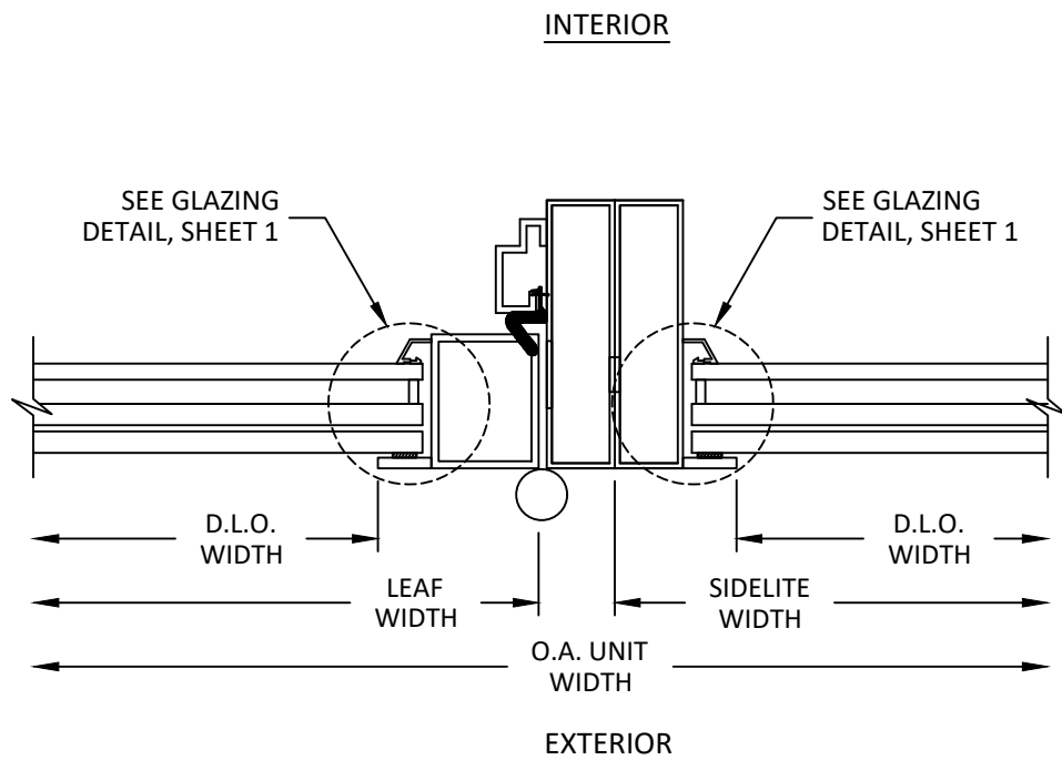
F 8 HORIZONTAL SECTION MULLION
