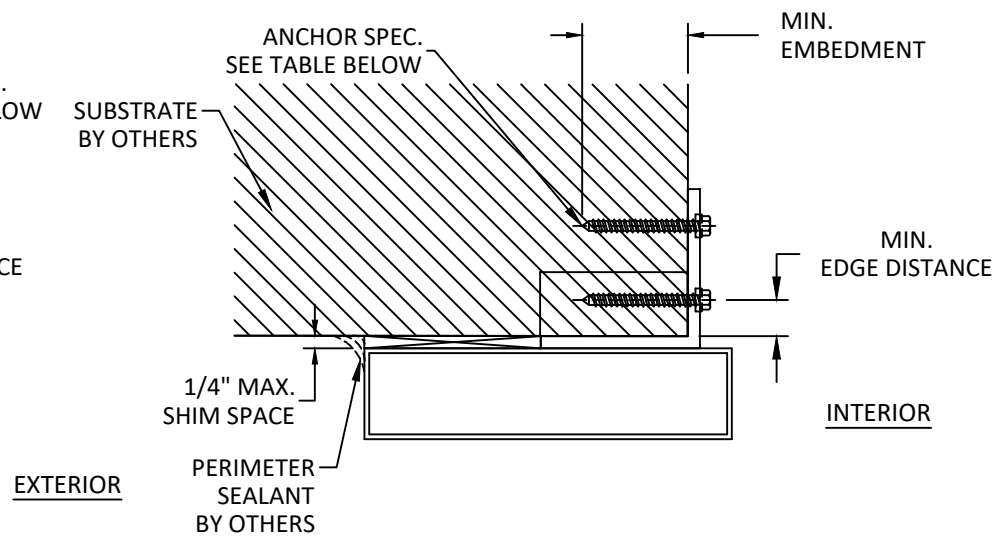
C 9 VERTICAL SECTION DOOR HEAD - TAB INSTALLATION
